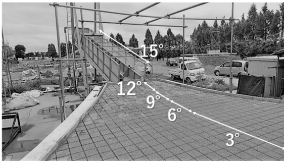
図-2. 実験水路 Fig.2 Experimental Flume
